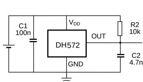
Typical Three-Wire Application Circuit
